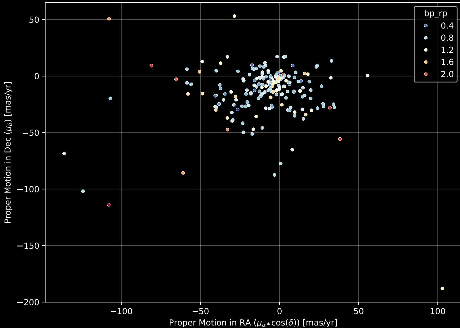
APOGEE DR17 Field: [177+49_MGA] Proper Motion Diagram (n= 201)
