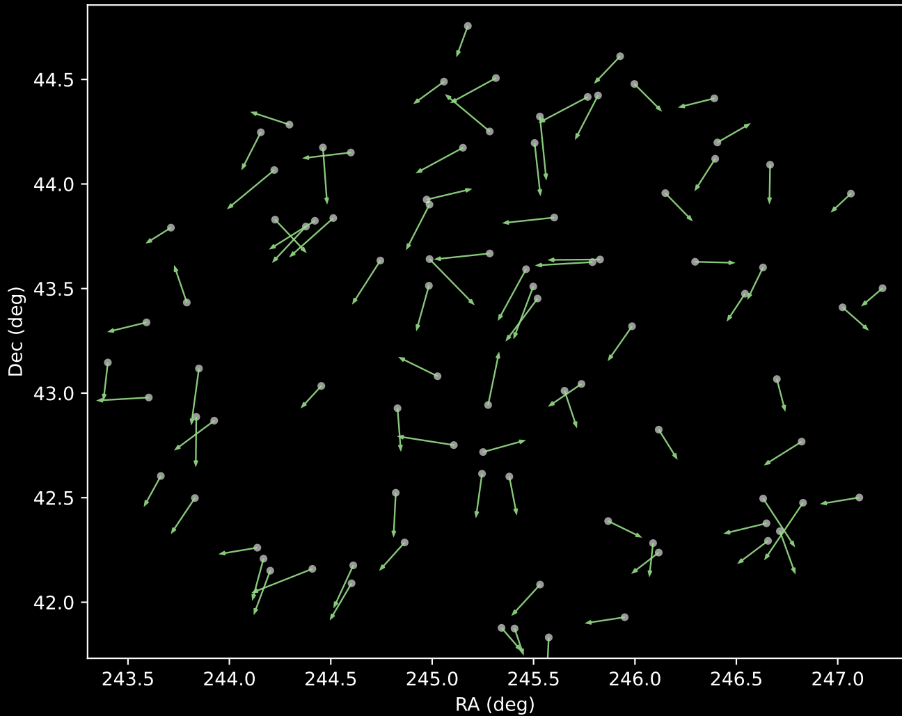
APOGEE DR17 Cluster 5 Proper Motion Vectors (n=89)
