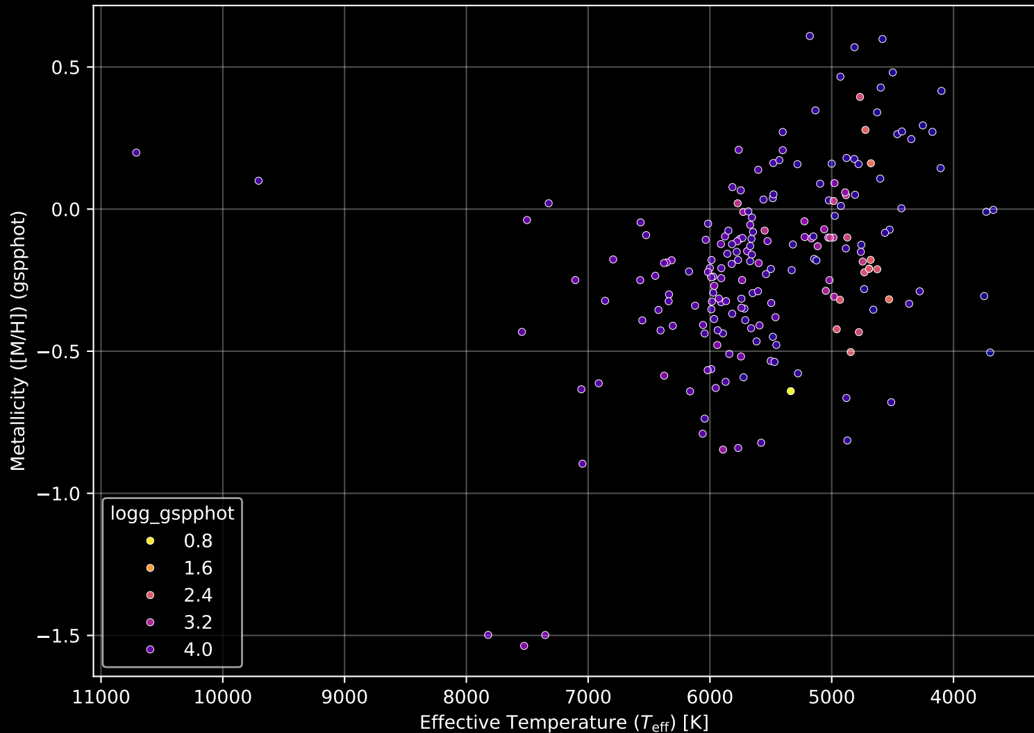
APOGEE DR17 Field: [177+49_MGA] Stellar Population Parameters (n= 201)
