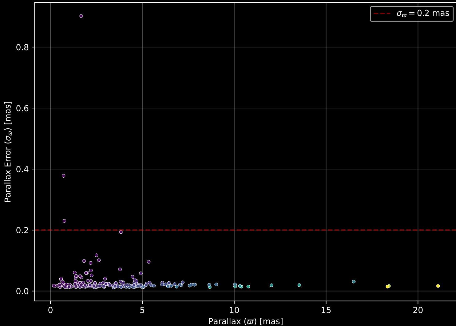
APOGEE DR17 Field: [177+49_MGA] Parallax Quality (n= 201)
