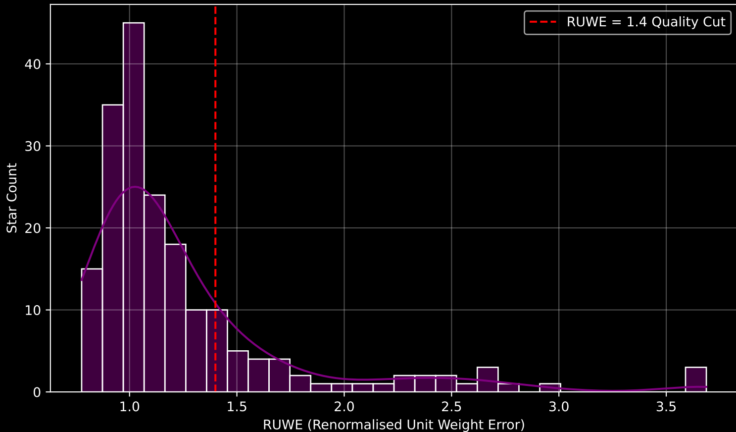
GAPOGEE DR17 Field [177+49_MGA] RUWE Distribution (n= 191)
