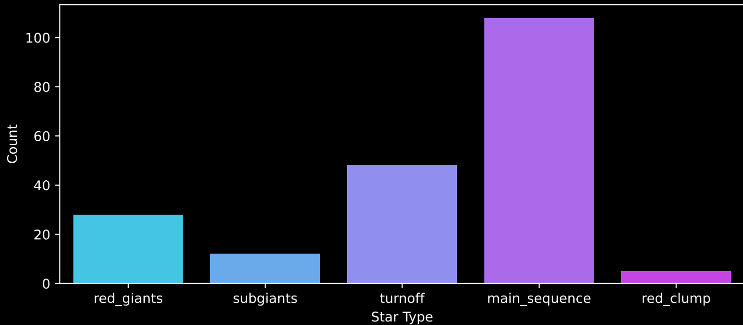
APOGEE DR17 Field: [177+49_MGA] Count plot of Star Type
